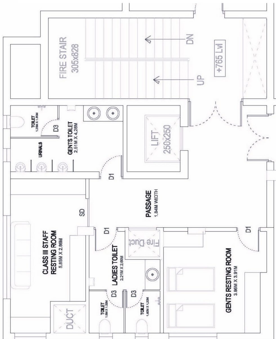
Passage Area- 2F- OB- Main Layout
