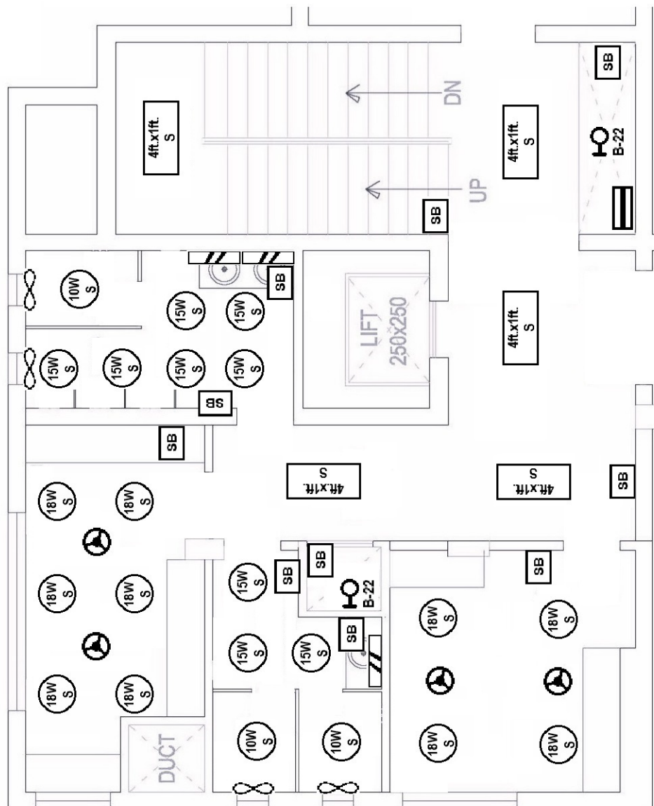
Passage Area- 2F- OB- Fittings
