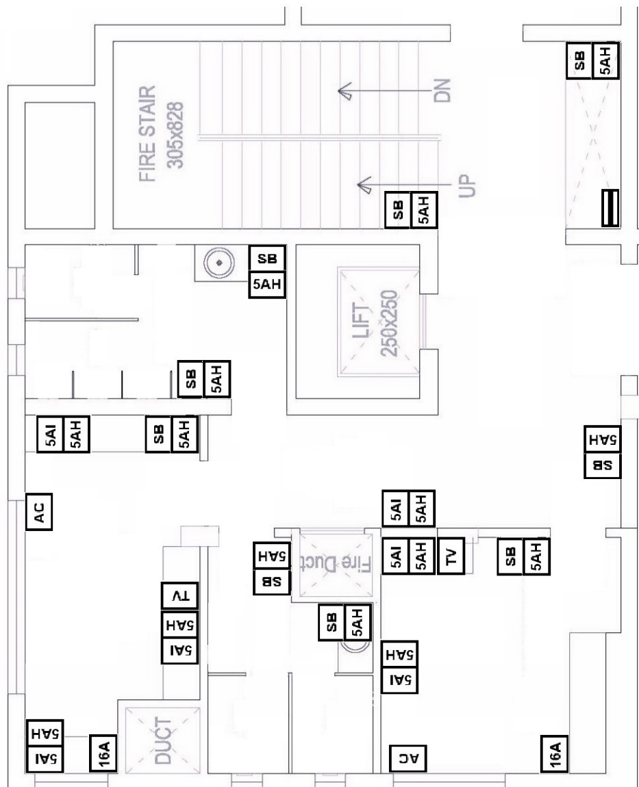
Passage Area- 2F- OB- Points
