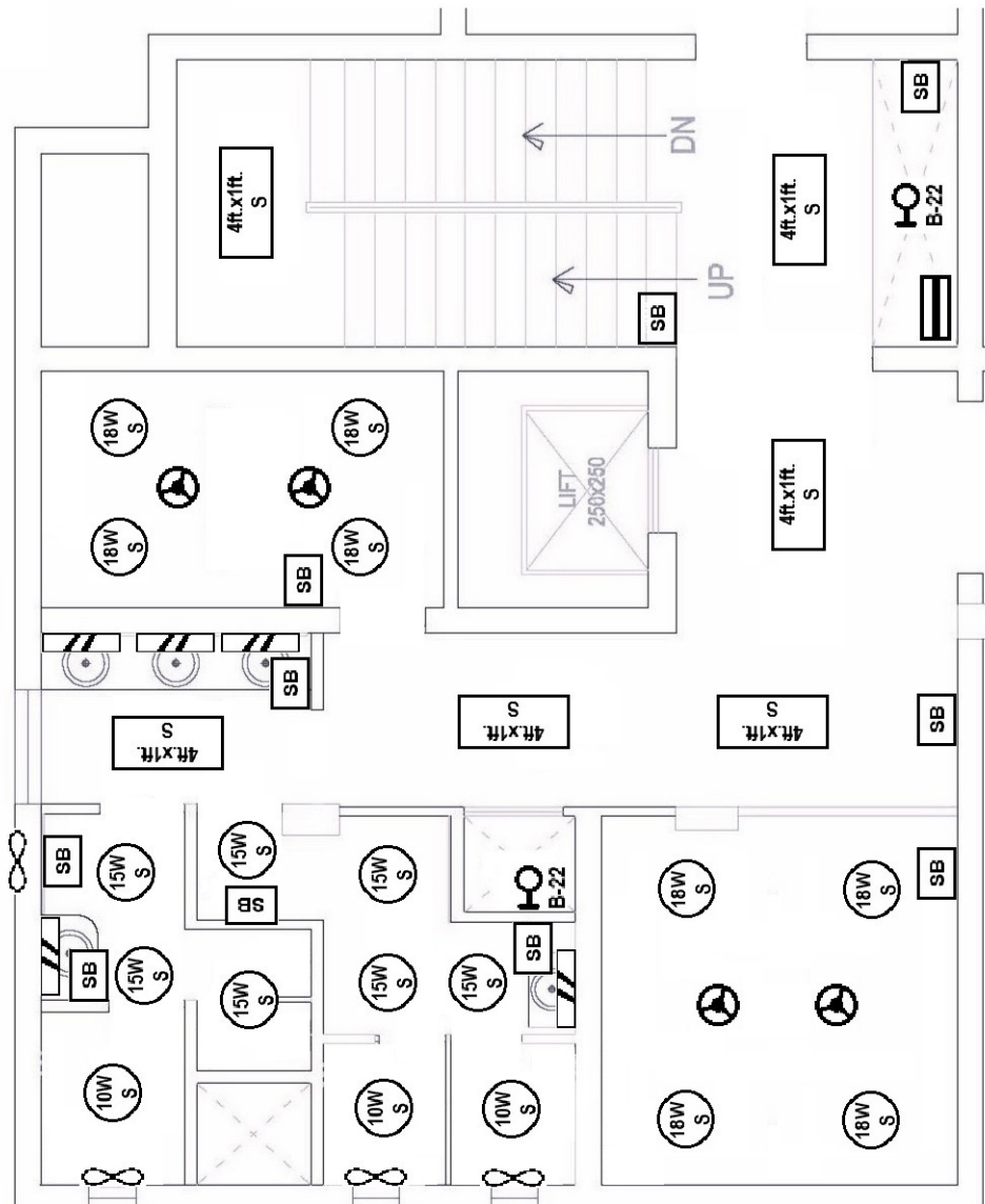
Passage Area- 3F- OB- Fittings
