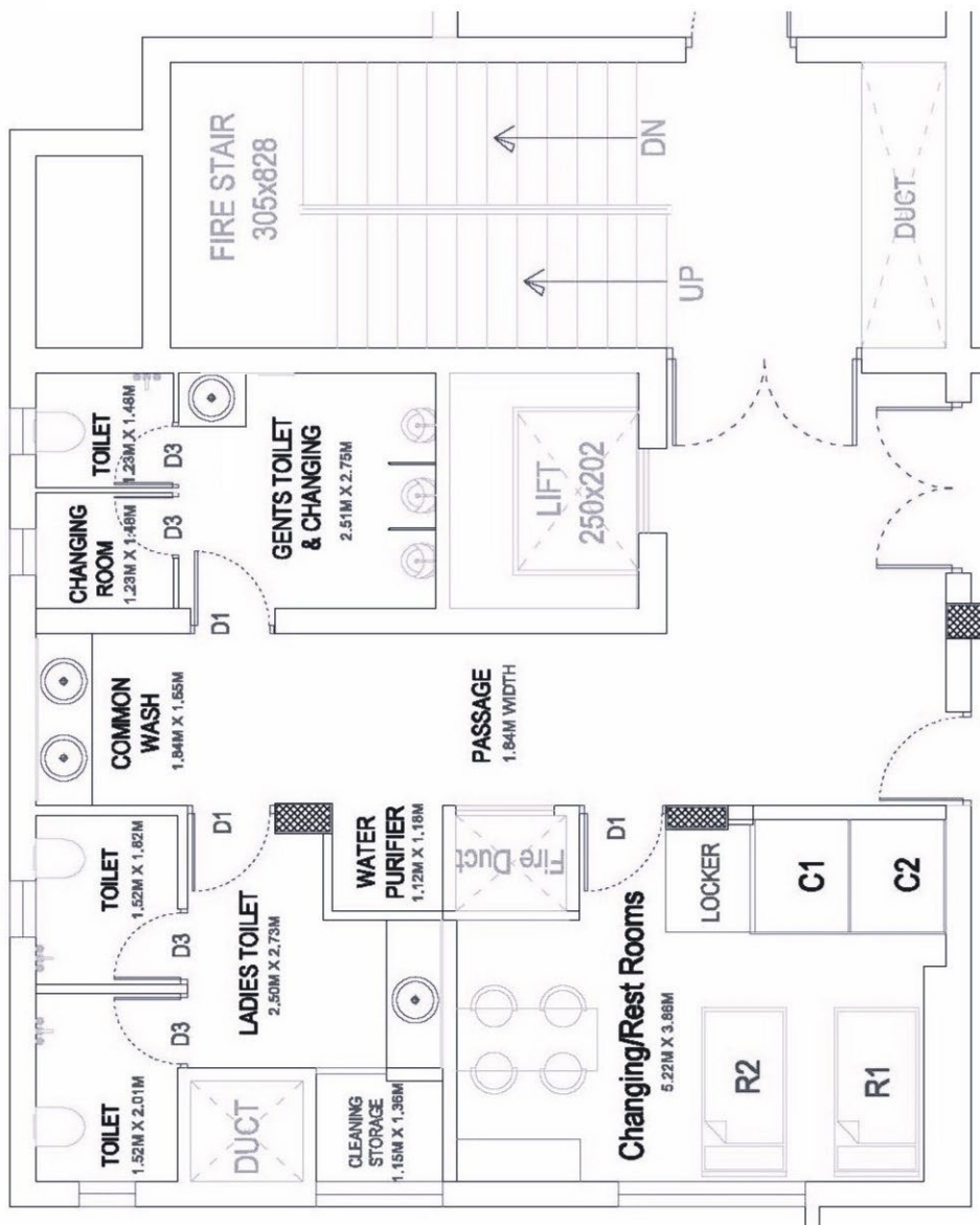
Passage Area- 1F- OB- Main Layout
