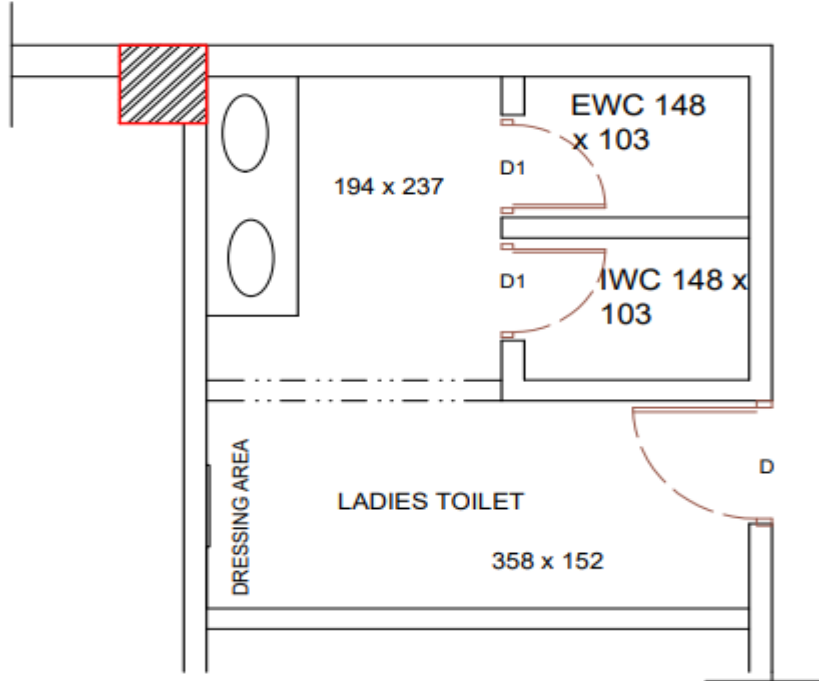
MAIN OFFICE - LAYOUT OF EXISTING LADIES WASHROOMS AT FIRST FLOOR
