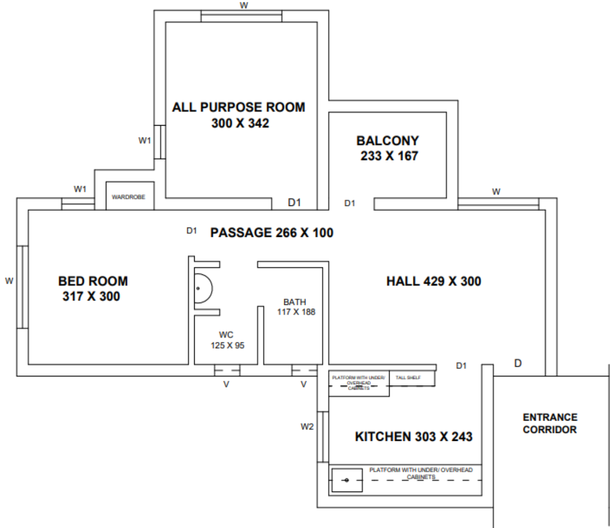
CLASS III FLAT AT THAMALAM TYPICAL LAYOUT
