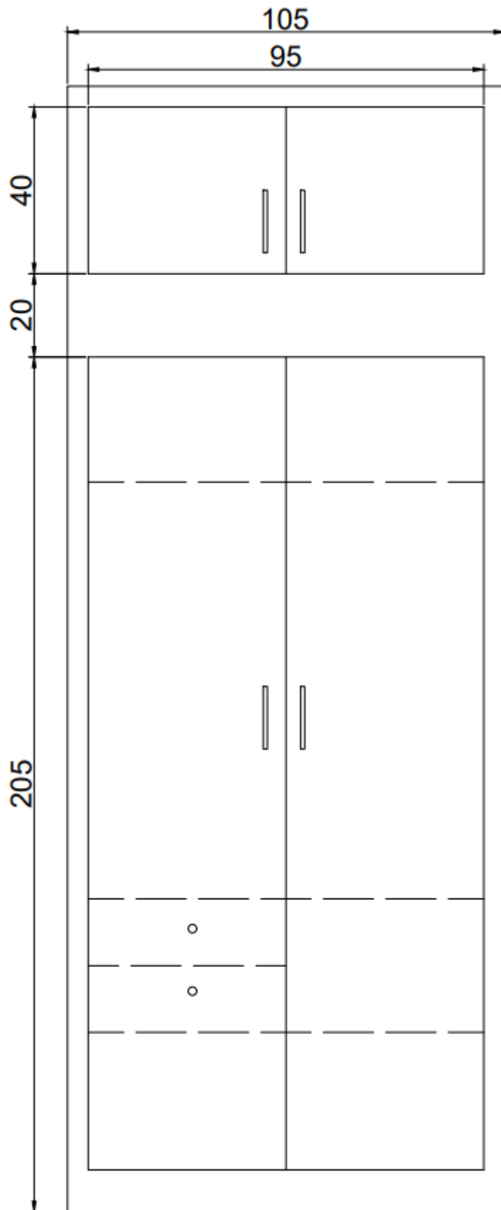
WARDRBE DETAILS
