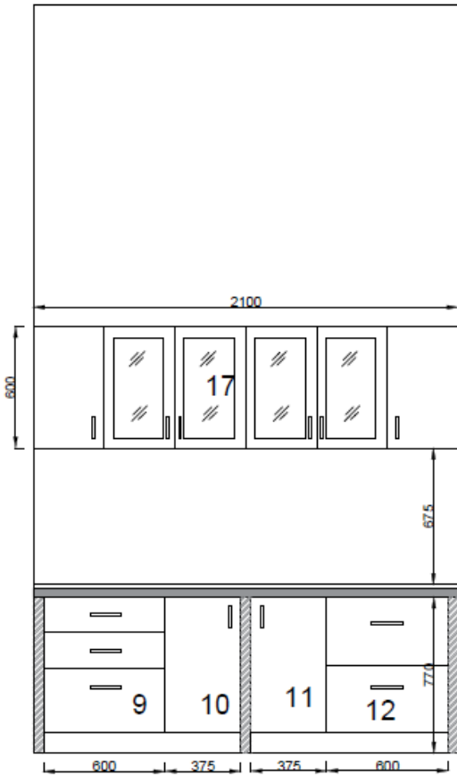
Elevation- C
