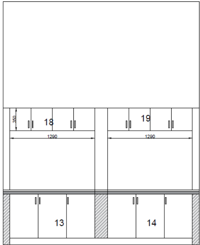
Elevation- E
