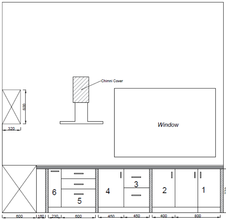
Elevation- A
