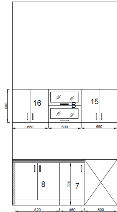
Elevation- D
